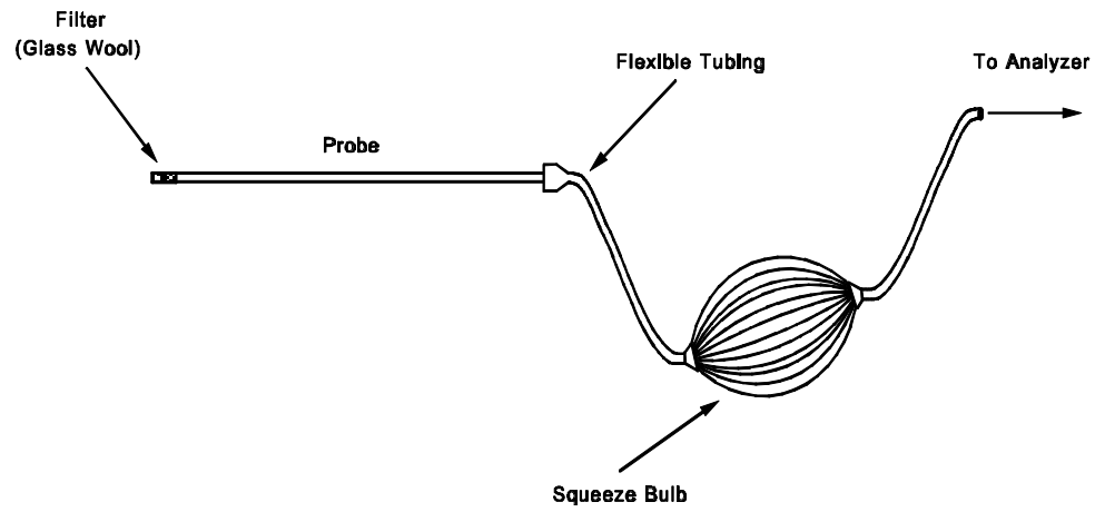
Figure 3-1. Grab-Sampling Train
